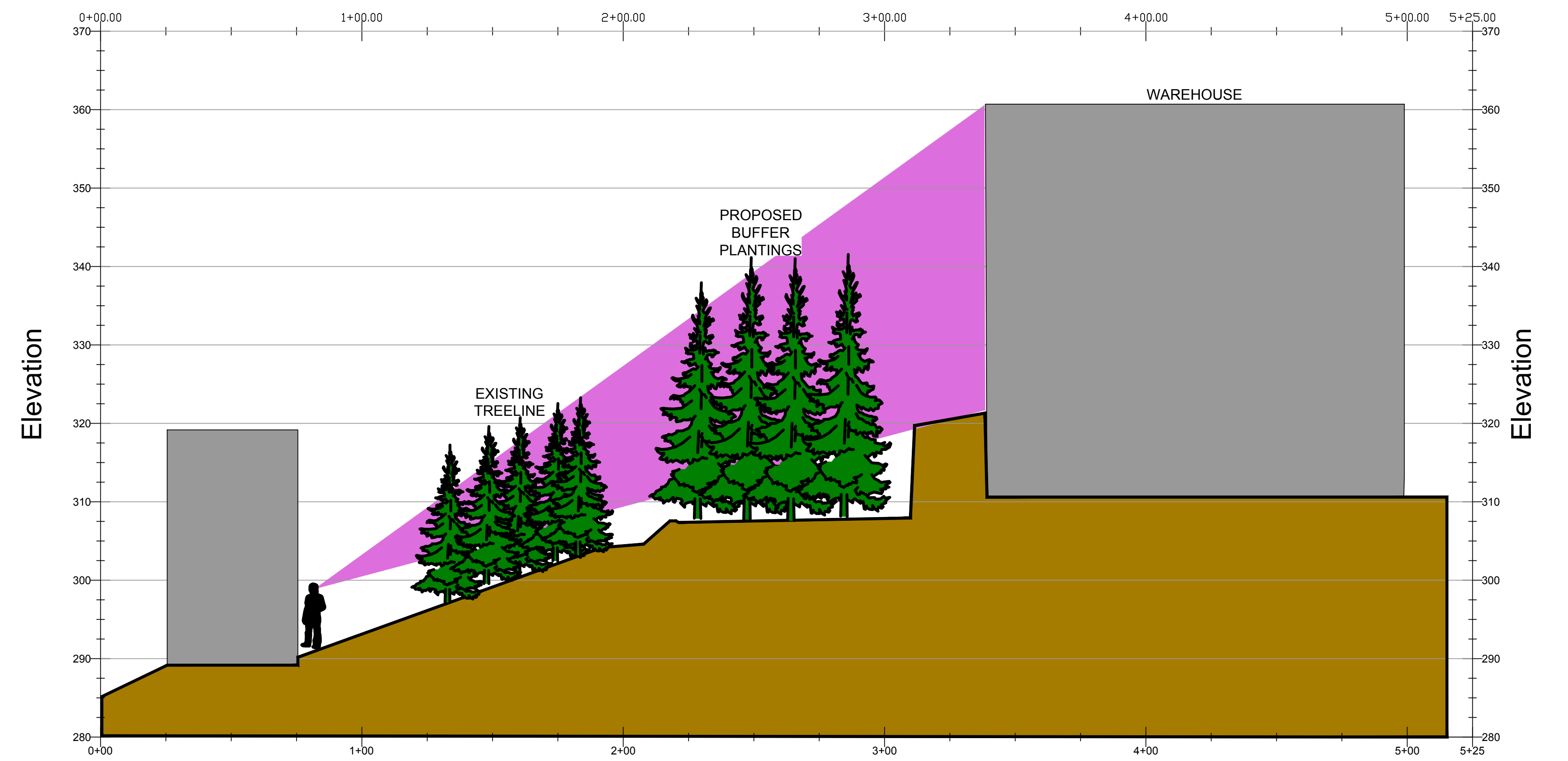
SECTION VIEW A-A
